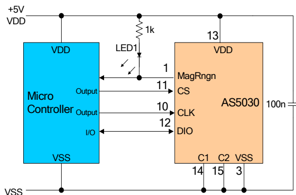
Figure 24: Magnetic field strength indicator
