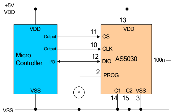
Figure 23: Analog OTP verification
