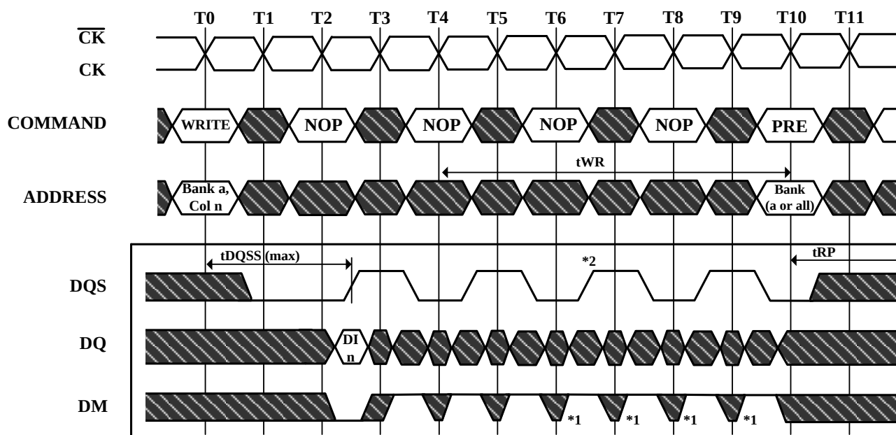
Figure 27. Write to Precharge Max tDQSS ODD Number of Data Interrupting
