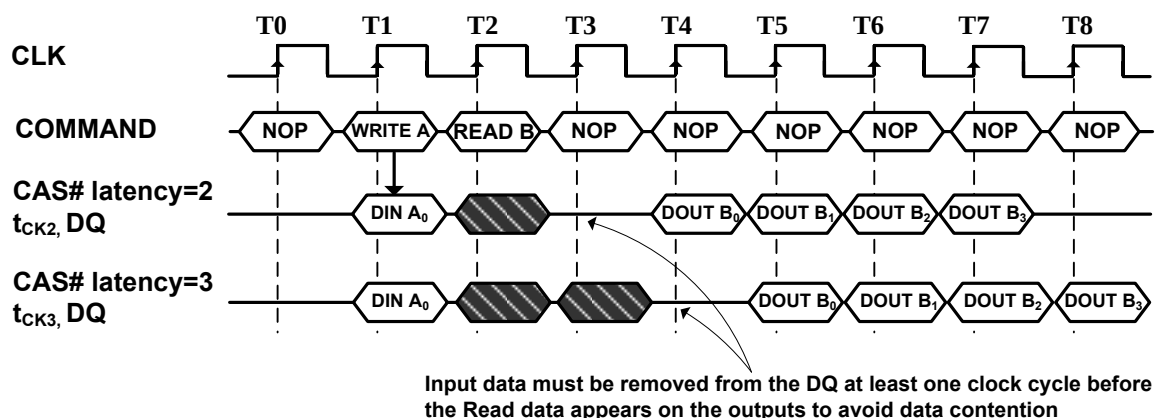
Figure 12. Write Interrupted by a Read (Burst Length = 4, CAS# Latency = 2, 3)
