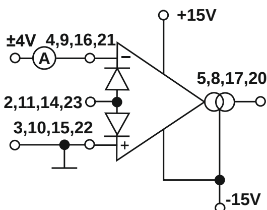
Differential Input Current Test Circuit
