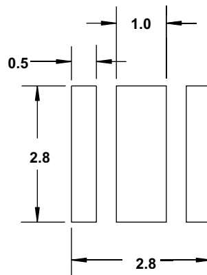
Figure 13: Recommended Soldering Land Pattern
