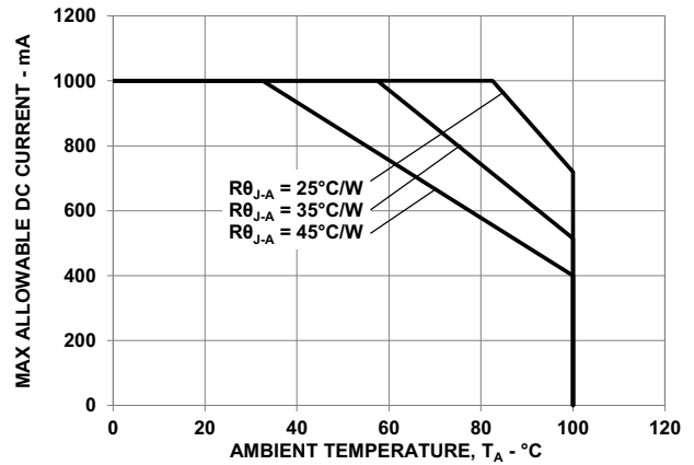
Figure 11: Maximum Forward Current vs. Ambient Temperature for ARE1-9x30
