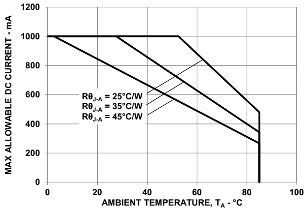
Figure 10: Maximum Forward Current vs. Ambient Temperature for ARE1-8x30
