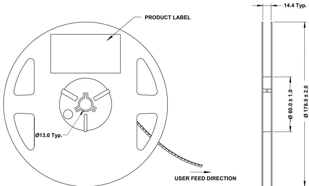
Figure 15: Reel Dimensions
