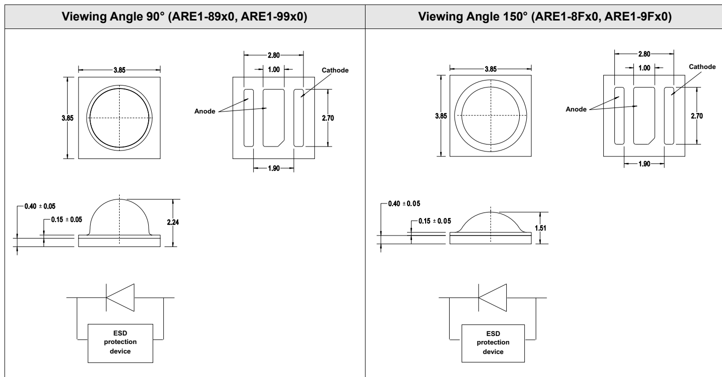
Figure 1: Package Drawing
