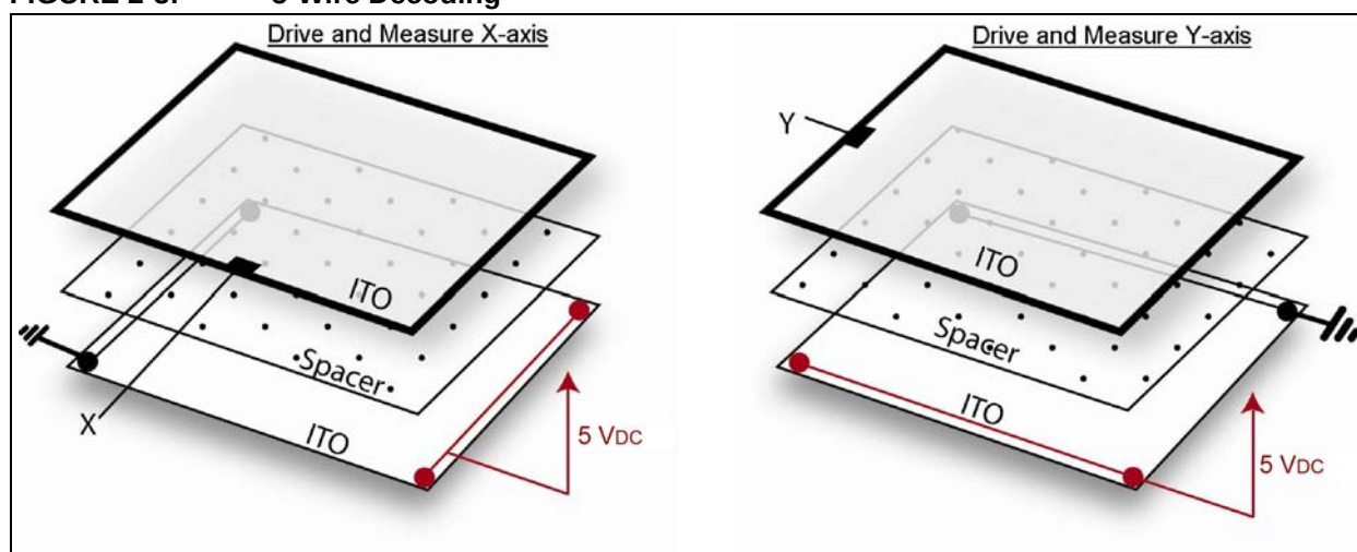
FIGURE 2-3: 5-Wire Decoding
