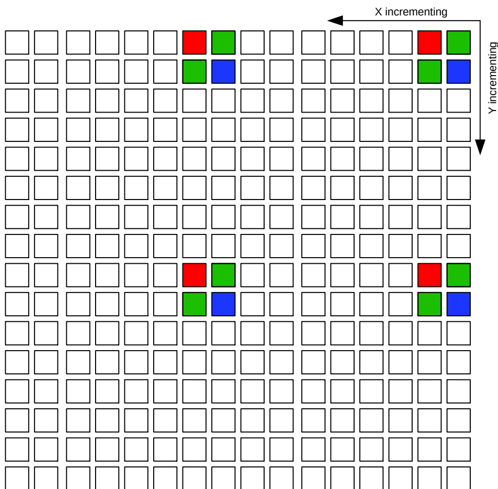
Figure 27. Skip4 Pixel Readout (x_odd_inc = 7, y_odd_inc = 7)
