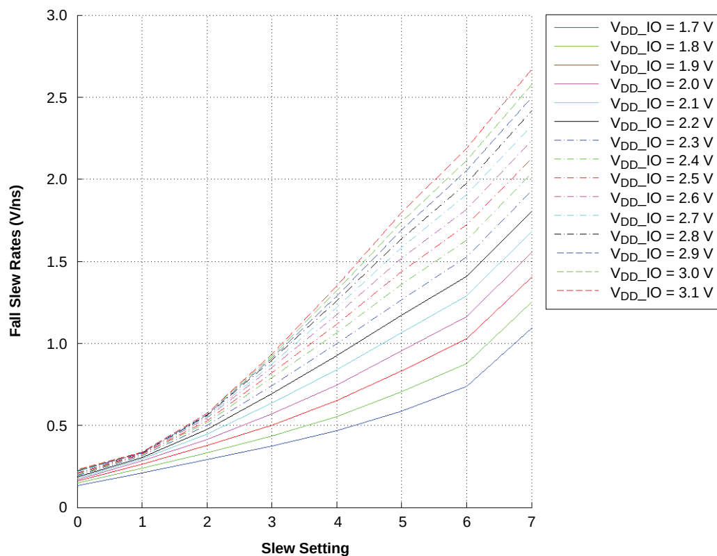
Figure 47. Fall Slew Rates (Cap Load = 25 pF)
