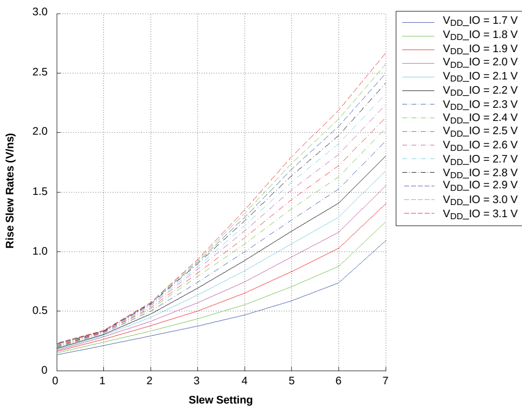
Figure 48. Rise Slew Rates (Cap Load = 25 pF)
