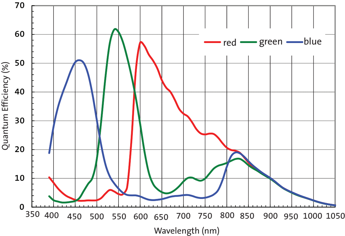
Figure 30: Quantum Efficiency – Color Sensor
