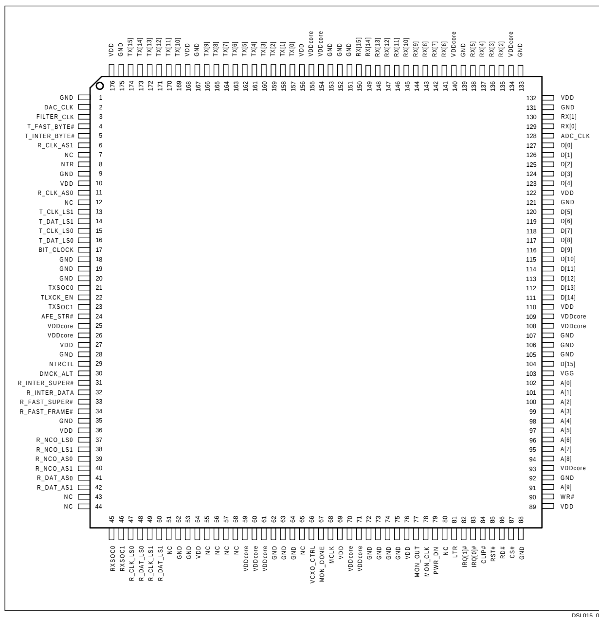
Figure 5. 11627 Pinout Diagram
