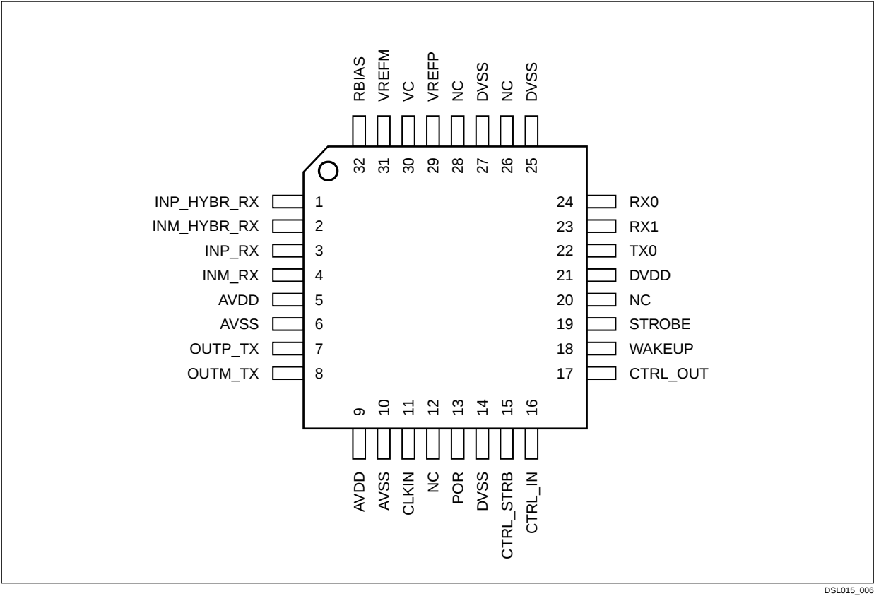
Figure 6. 20431 Pinout Diagram
