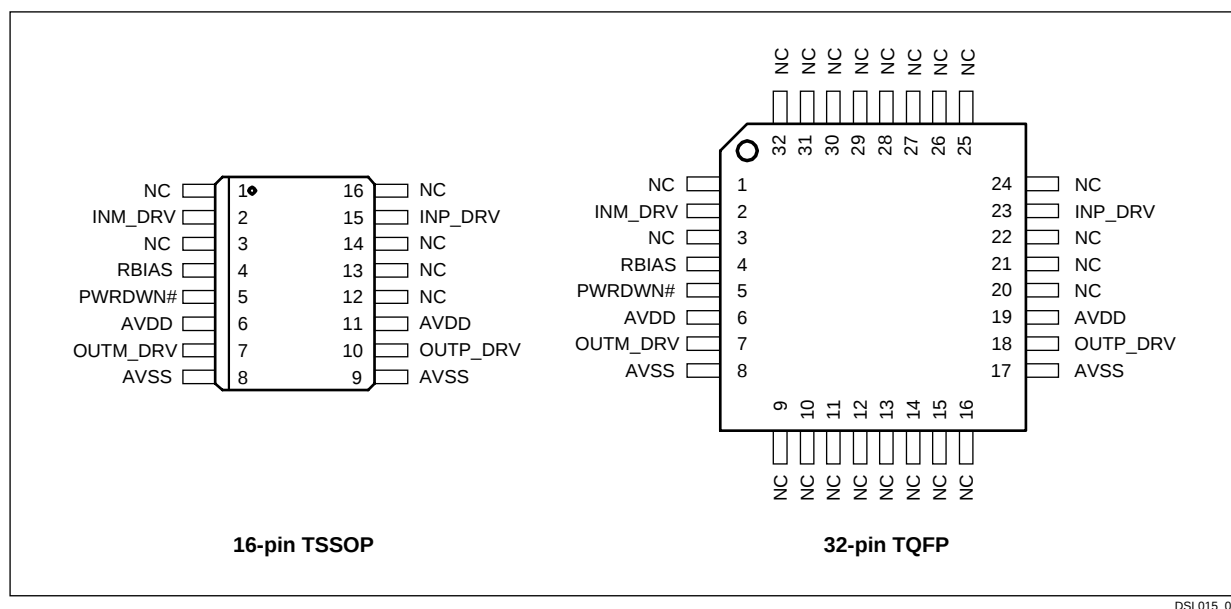
Figure 7. 20441 Pinout Diagrams
