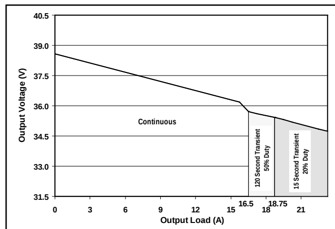
Figure 6: 36 V OUT droop characteristic.
