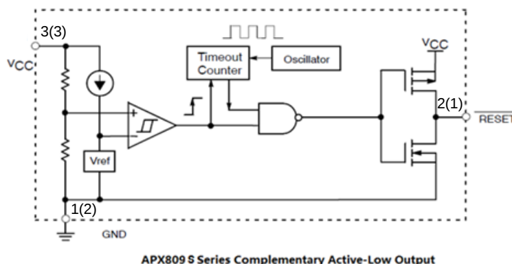
APX809S Series Complementary Active-Low Output
