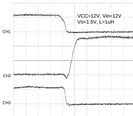
UGATEFalling
