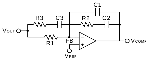
Figure 5. Compensation Network
