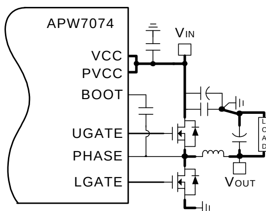
Figure 7. Layout Guidelines
