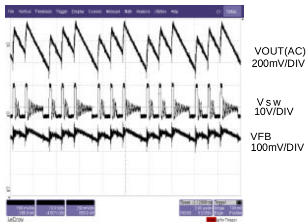
Burst Mode Operation
