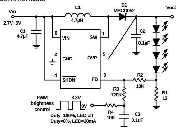
Fig. 5 Brightness Control by a filtered PWM signal
