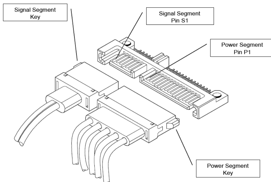
Figure 1-2 Pin Assignments
