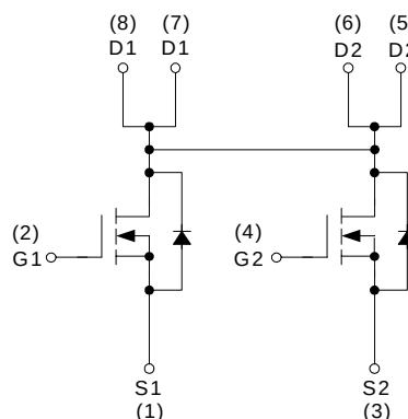
N-Channel MOSFET
