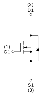
N-Channel MOSFET
