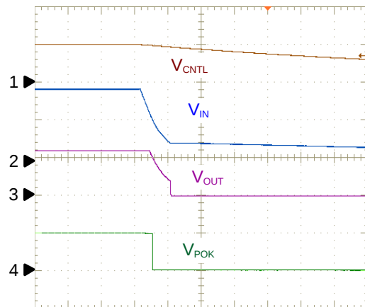
Power Off
