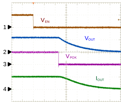
Shutdown
