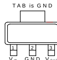
SOT-223 (Top View) APL5509R
