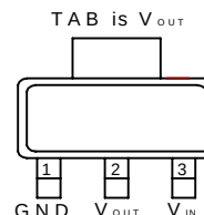
SOT-223 (Top View) APL5508R
