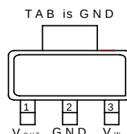
SOT-223 (Top View) APL5509
