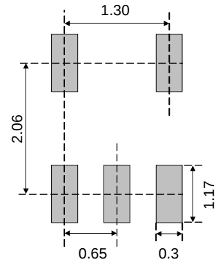
SC-70-5
