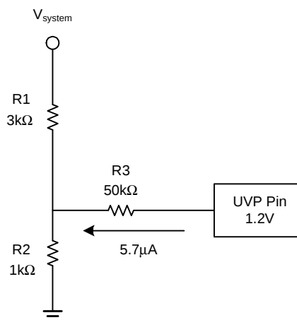
Figure2. Under-Voltage Protection
