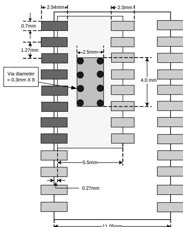
Figure 5. APA2603 SOP-16P & APA2603A SOP-24co-layout Land Pattern Recommendation
