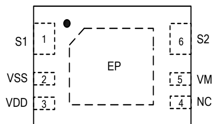
U-DFN2030-6
