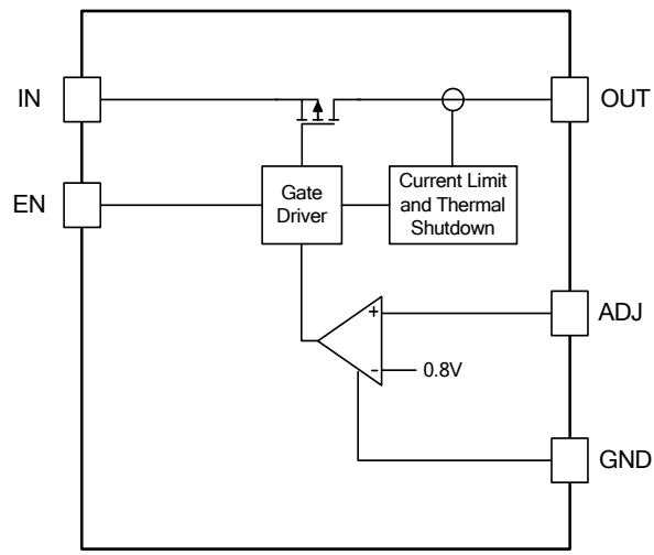
Adjustable Version
