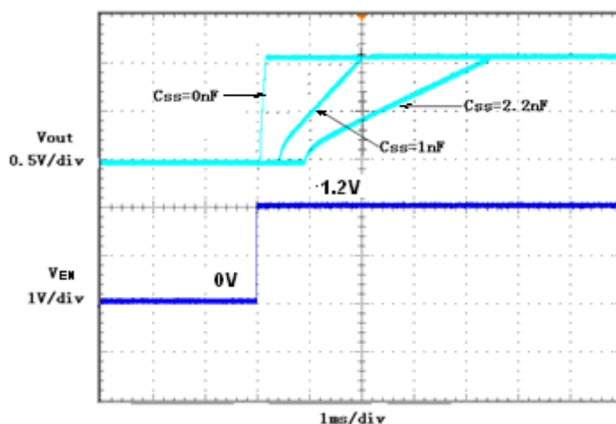
Figure 2. Turn-On Response
