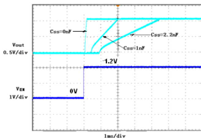
Figure 2. Turn-On Response
