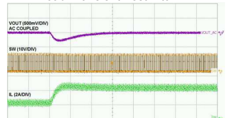
Load Transient Test 2 to 4A
