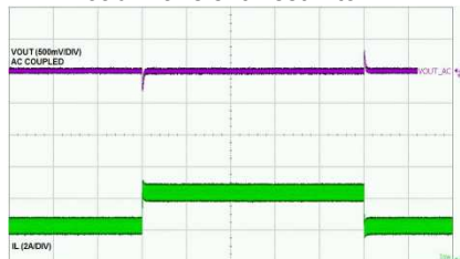
Load Transient Test 2 to 4A
