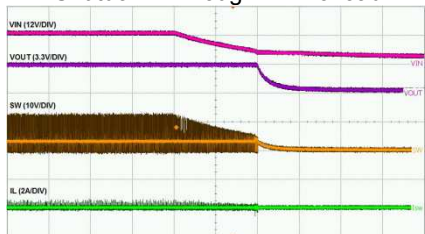
Shutdown Through Vin no load
