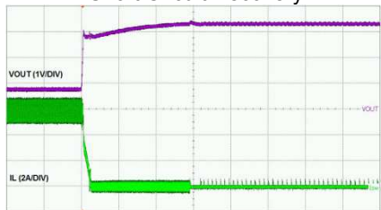
Short Circuit Recovery
