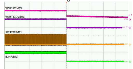
Shutdown Through Vin 4A Load
