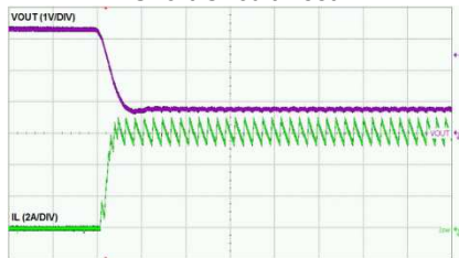
Short Circuit Test
