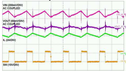
Steady State Test 4A
