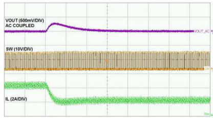
Load Transient Test 4A to 2A
