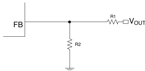
Figure 3 Feedback Divider Network
