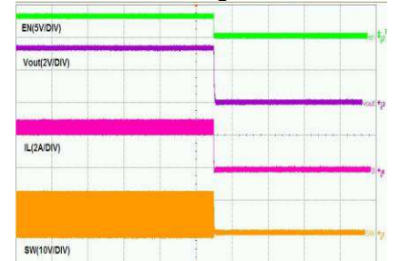
Shutdown Through Enable 2A
