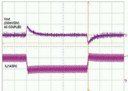
Load Transient Test 1.0A to 2.0A
