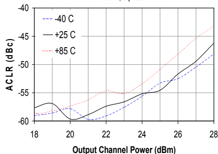
ACLR vs. Channel Power
