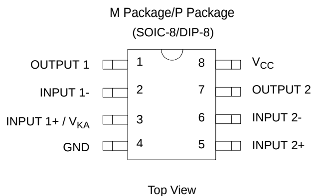
Figure 2. Pin Configuration of AP4310
