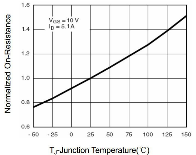
Figure 8 Drain-Source On-Resistance
