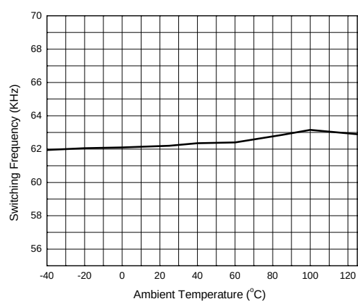
Figure 8. Switching Frequency vs. Ambient Temperature
