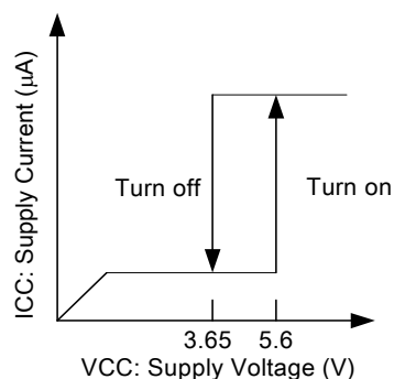
Figure 13. 5.6/3.65V UVLO Threshold of AP3710
