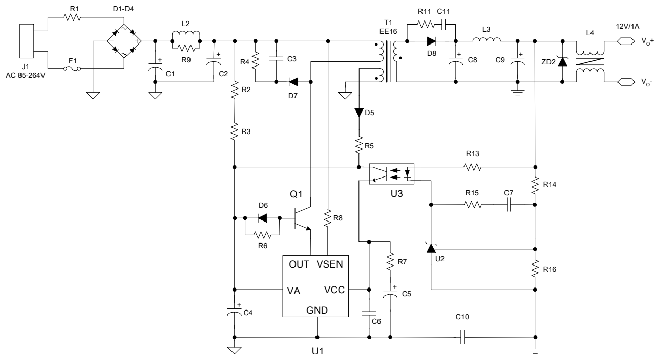
Figure 19. 12V/1A Adapter
