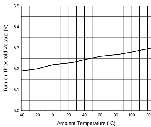
Figure 12. Turn on Voltage vs. Ambient Temperature
