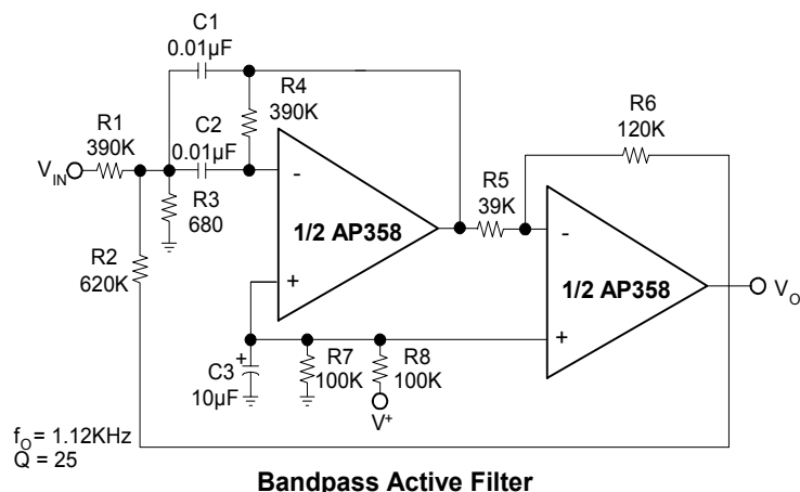
Bandpass Active Filter
