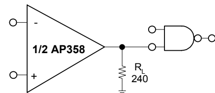
Driving TTL
