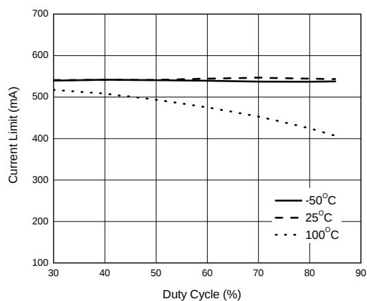
Figure 15. Current Limit vs. Duty Cycle
