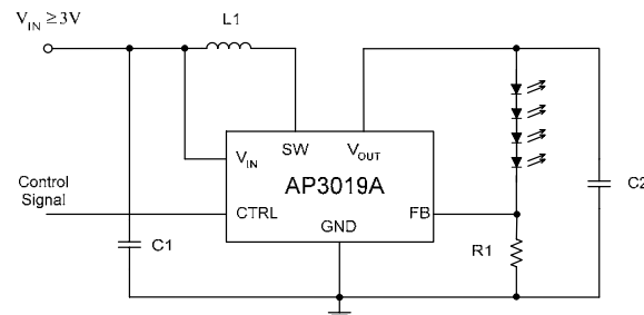
Figure 18. Typical Application Circuit to Decide R1
