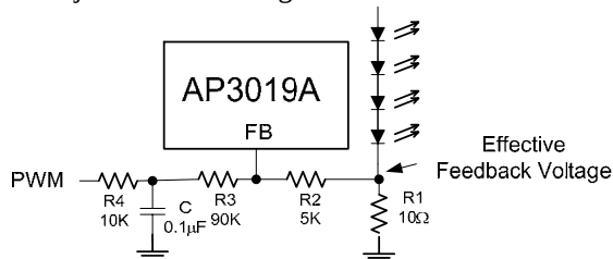
Figure 22. Dimming Control Using a Filtered PWM Voltage
