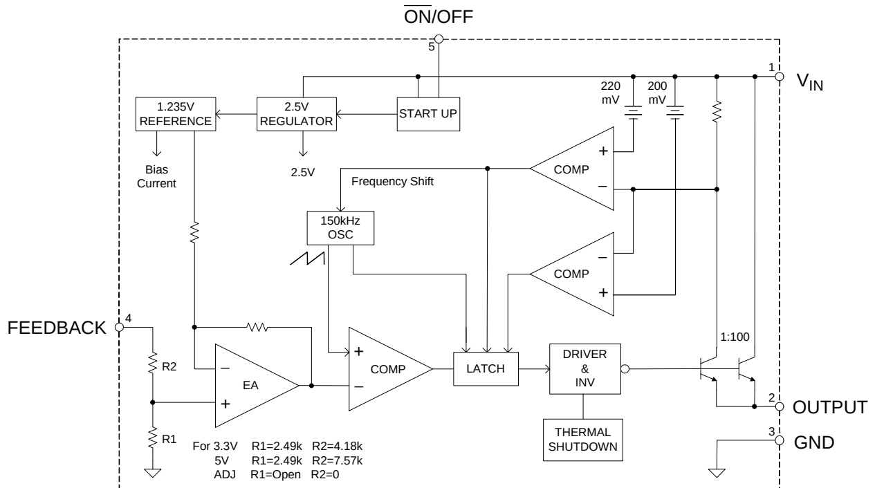
Figure 3. Functional Block Diagram of AP3001
