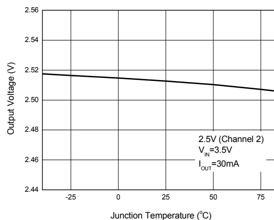
Figure 21. Output Voltage vs. Junction Temperature
