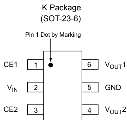
Figure 2. Pin Configuration of AP2401 (Top View)
