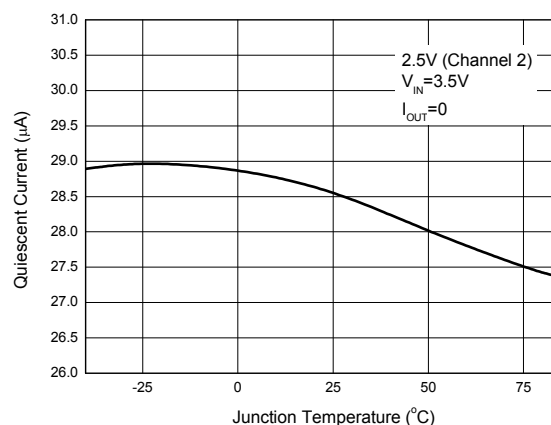
Figure 29. Quiescent Current vs. Junction Temperature
