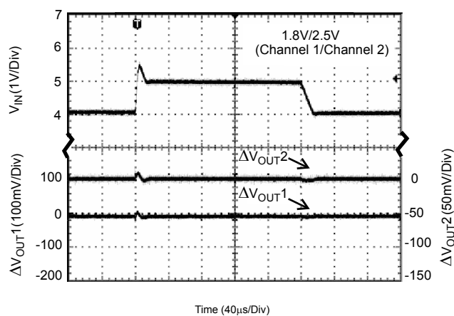
Figure 36. Line Transient (Conditions: channel 1 and 2 on, I_{OUT}=30\text{mA} , C_{IN}=C_{OUT}=1\mu\text{F} )
