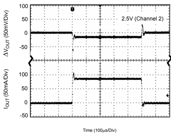
Figure 38. Load Transient (Conditions: I_{OUT}=10 to 100\text{mA} , C_{IN}=C_{OUT}=1\mu\text{F} )
