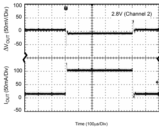
Figure 39. Load Transient (Conditions: I_{OUT}=10 to 100\text{mA} , C_{IN}=C_{OUT}=1\mu\text{F} )
