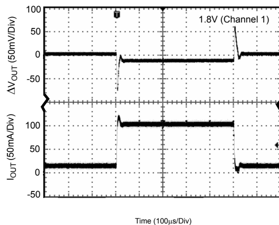
Figure 37. Load Transient (Conditions: I_{OUT}=10 to 100\text{mA} , C_{IN}=C_{OUT}=1\mu\text{F} )
