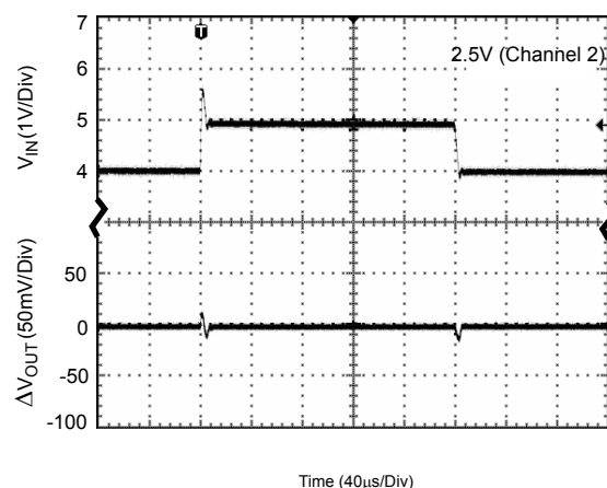
Figure 33. Line Transient (Conditions: I_{OUT}=30\text{mA} , C_{IN}=100\text{nF} , C_{OUT}=1\mu\text{F} )
