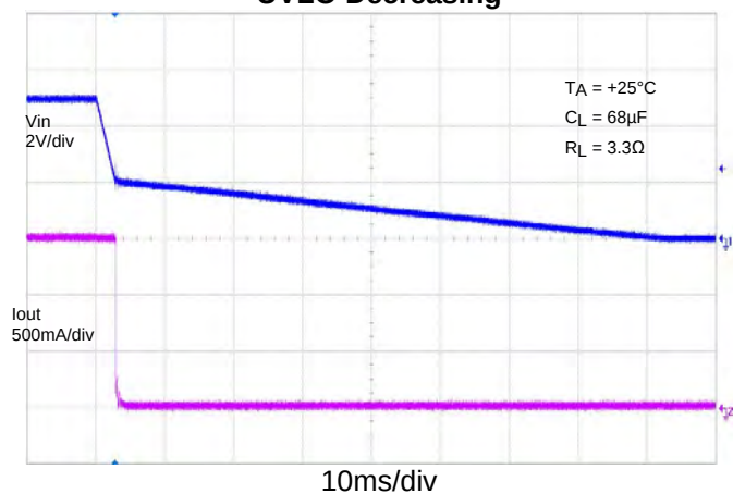
UVLO Decreasing
