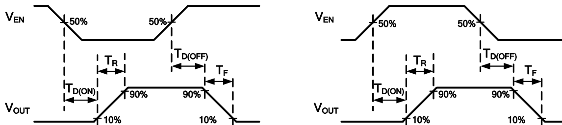
Figure 1 Voltage Waveforms: AP2181 (left), AP2191 (right)
