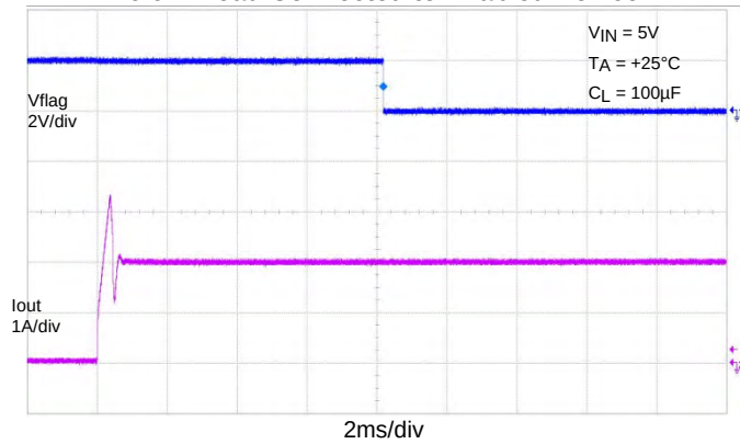
0.6 \Omega Load Connected to Enabled Device
