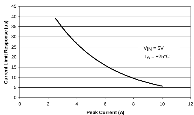
Current Limit Response vs Peak Current
