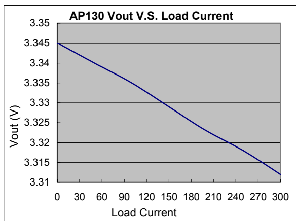
Vout V.S. Load Current
