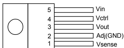
TO220-5L
