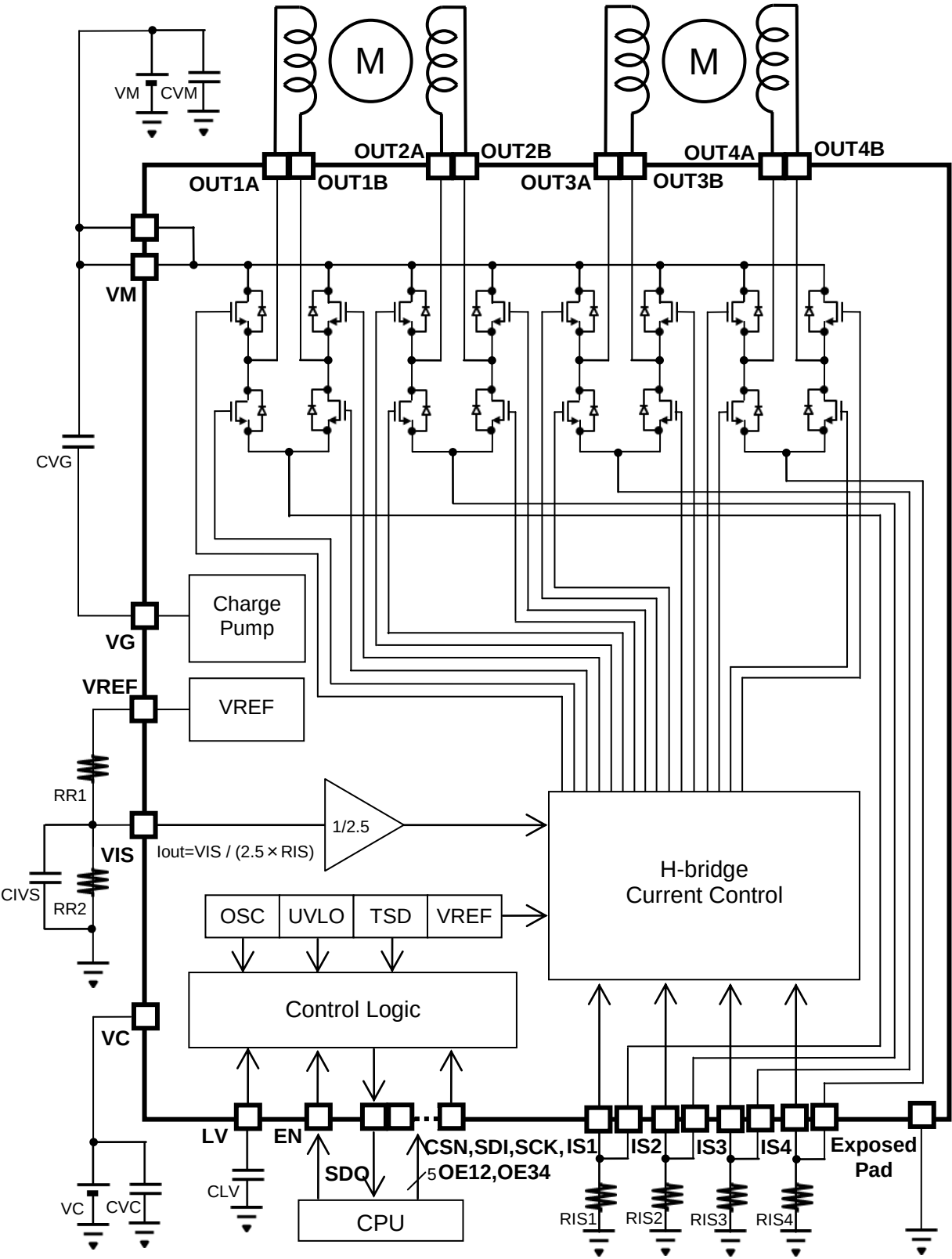
Figure 1. Block Diagram
