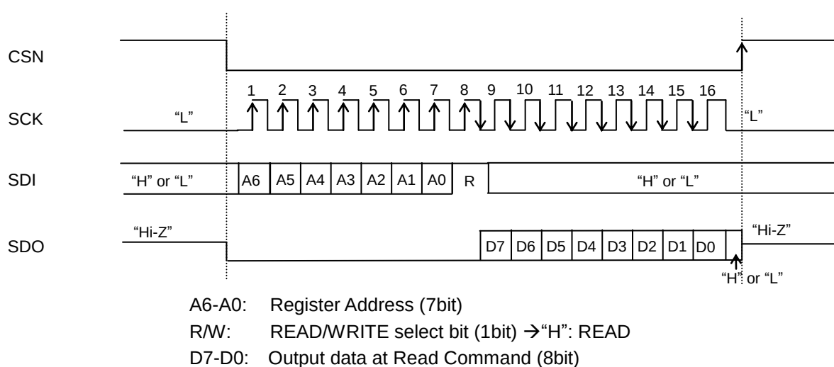
Figure 5. Serial Control Interface Timing (read mode)
