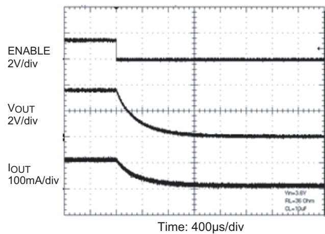
Turn-Off Timing
