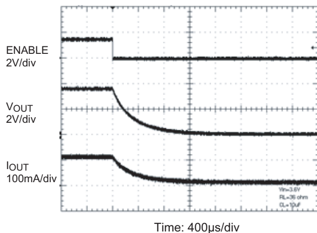
Turn-Off Timing
