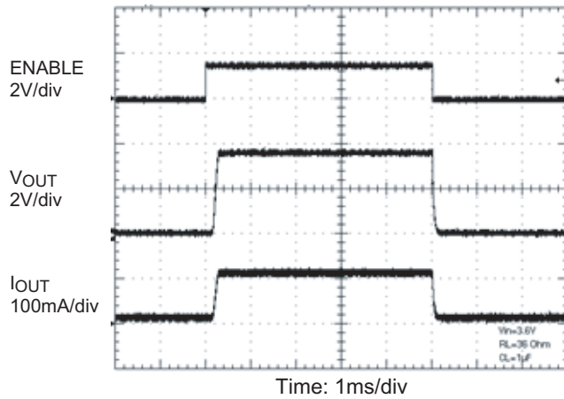
Turn-On/Turn-Off Timing
