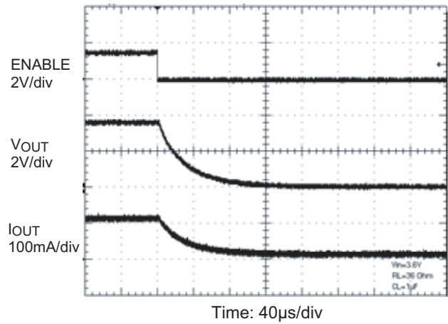
Turn-Off Timing
