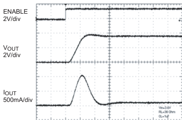
Turn-On Timing
