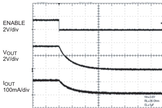
Turn-Off Timing
