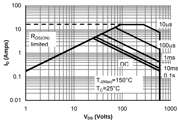
Figure 9: Maximum Forward Biased Safe Operating Area for AOT4N60 (Note F)
