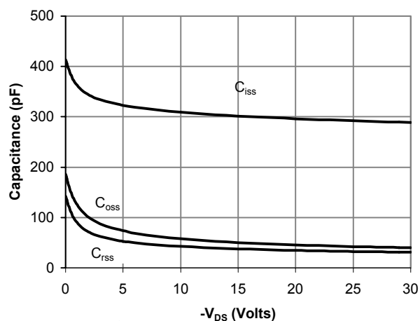
Figure 8: Capacitance Characteristics 370
