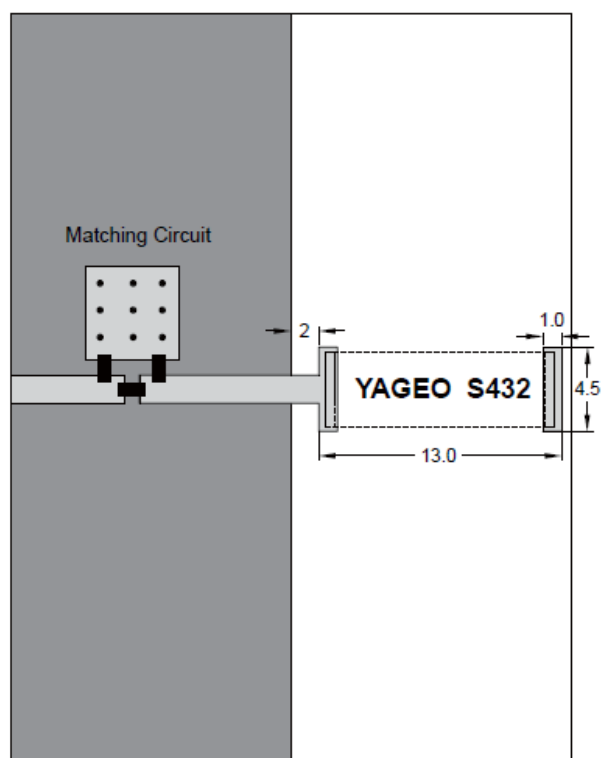
Fig. 3 Details of soldering Pad
