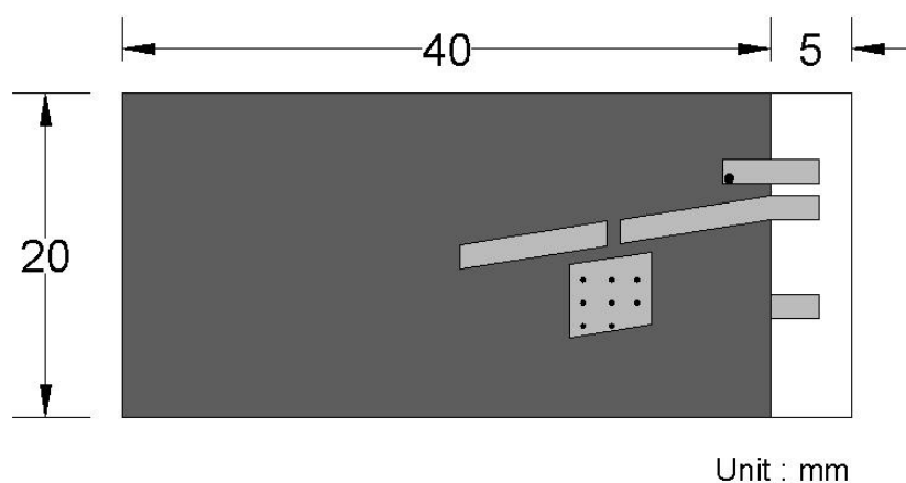
Fig. 2 Outlook and dimension of evaluation board
