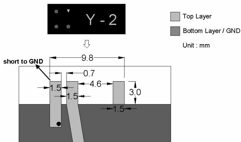
Fig. 3 Details of soldering Pad
