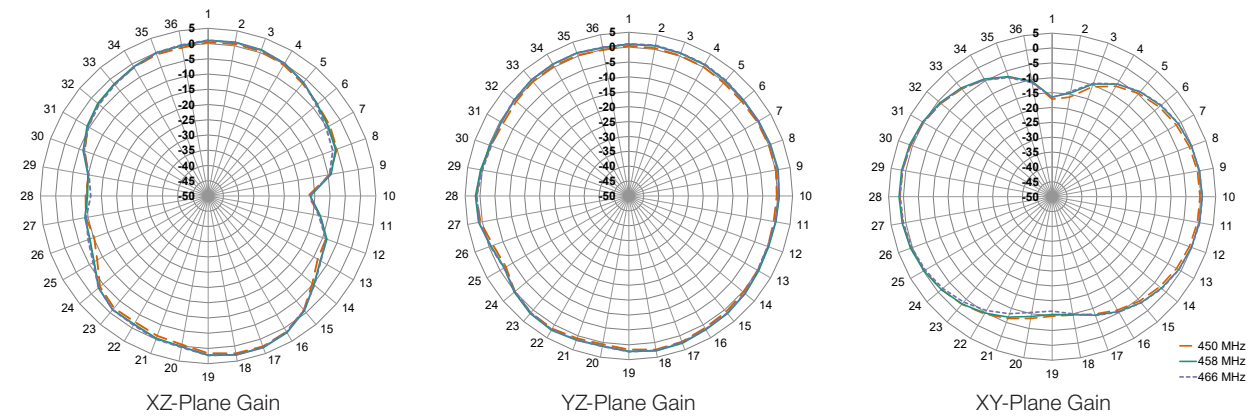
Figure 8. Radiation Patterns for PW 450 MHz Antenna
