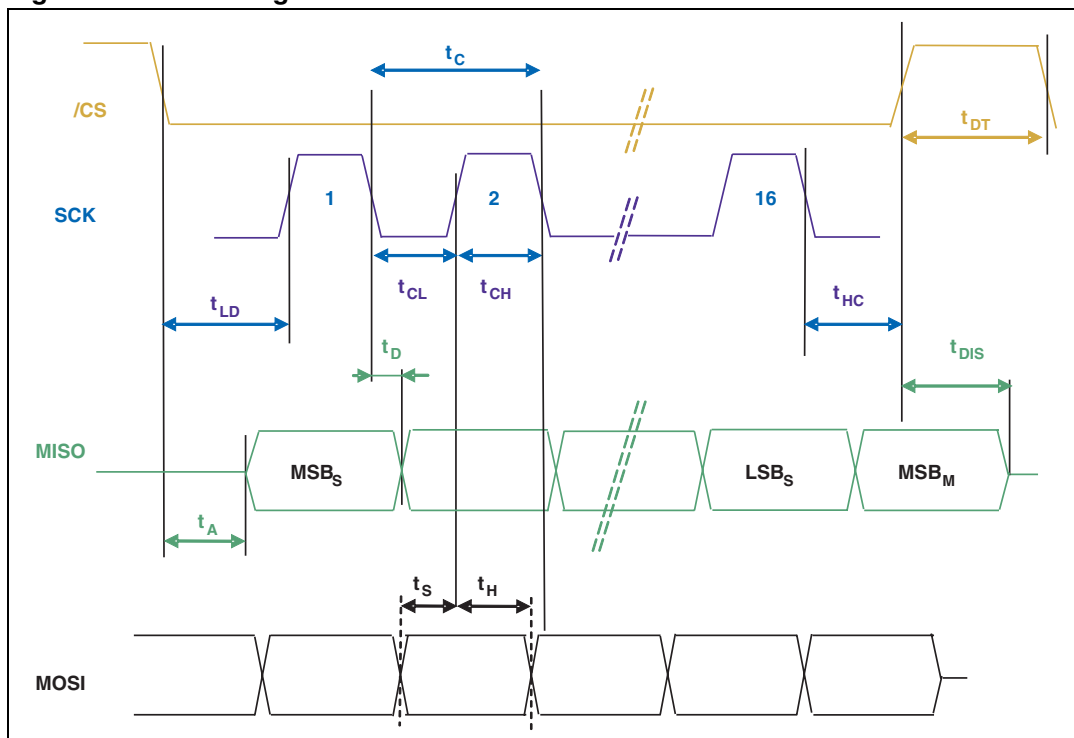
Figure 27. SPI timing definition.
