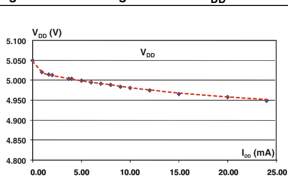
Figure 19. Load regulation with V_{DD} booster
