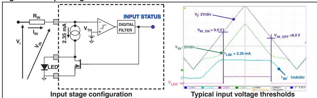
Figure 6. Input stage
