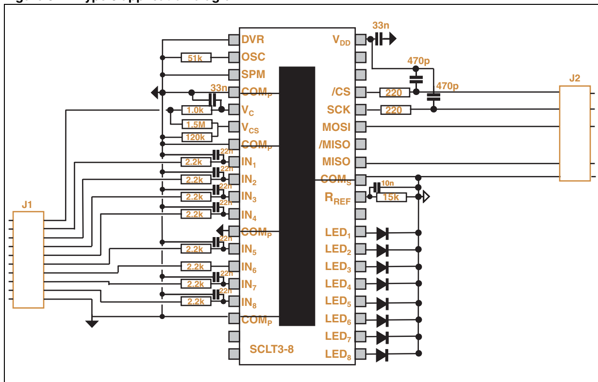
Figure 31. Type 3 application diagram
