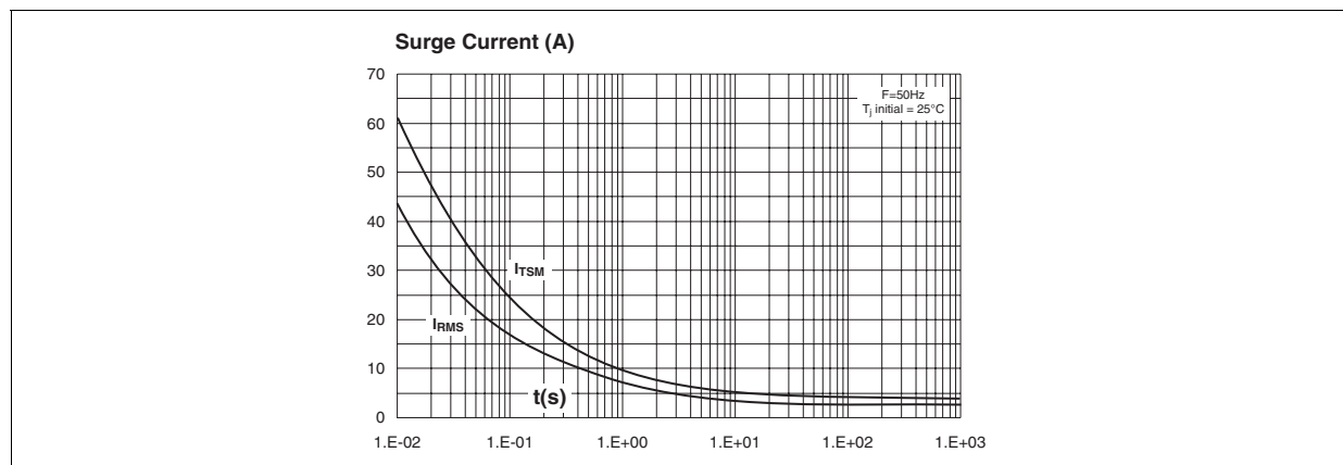
Figure 6: I_{TSM} and I_{RMS} capability versus surge duration
