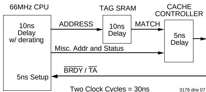
Figure 7. Conventional Tag RAM Usage - Chip Set in \overline{\text{BRDY}}/\overline{\text{TA}} Critical Path
