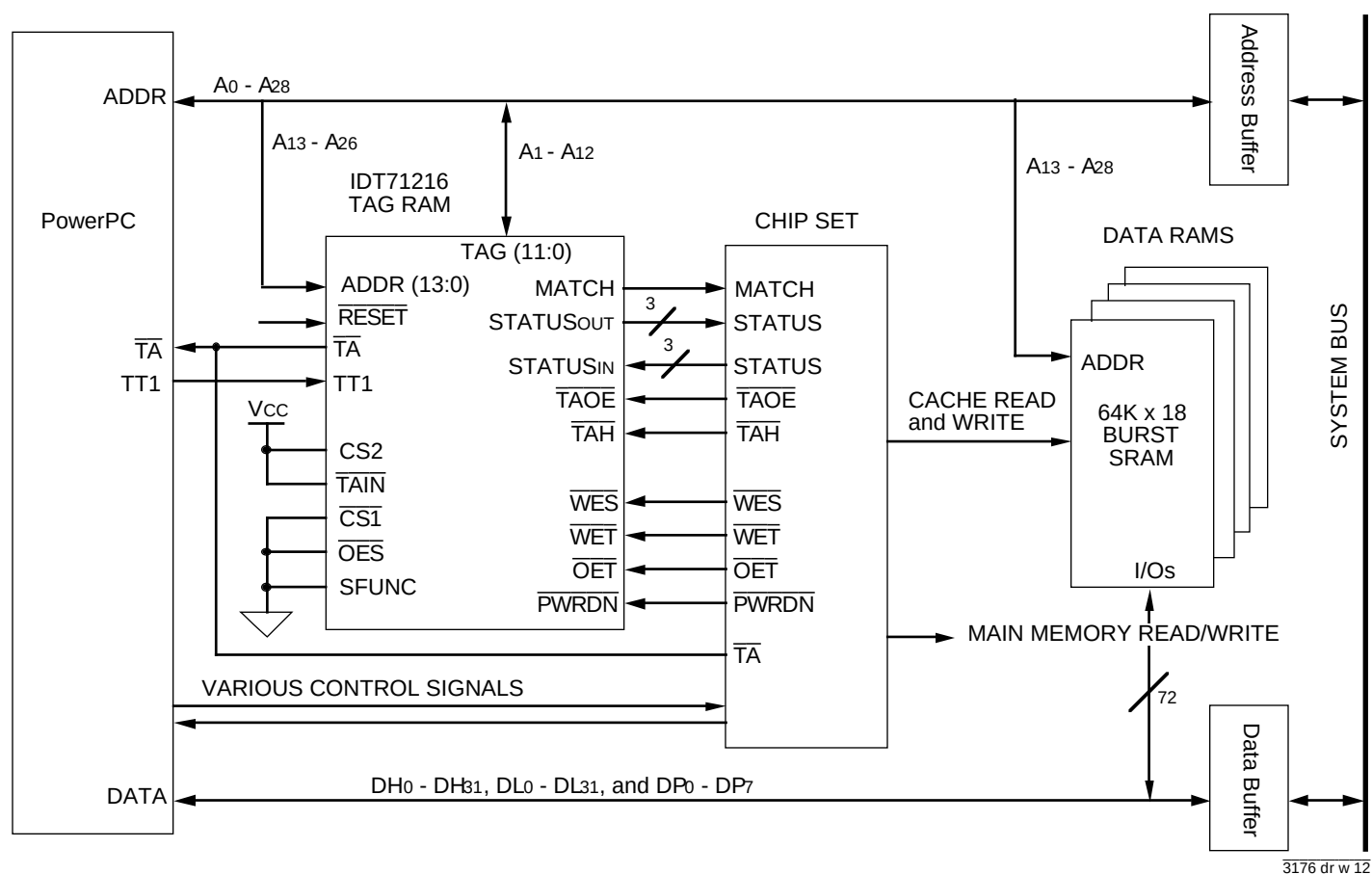
Figure 12: PowerPC / 71216 Example of 512 KB Cache
