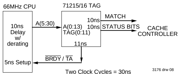
Figure 8. 71215/16 \overline{\text{BRDY}}/\overline{\text{TA}} Timing - Chip Set Removed from the Critical Path
