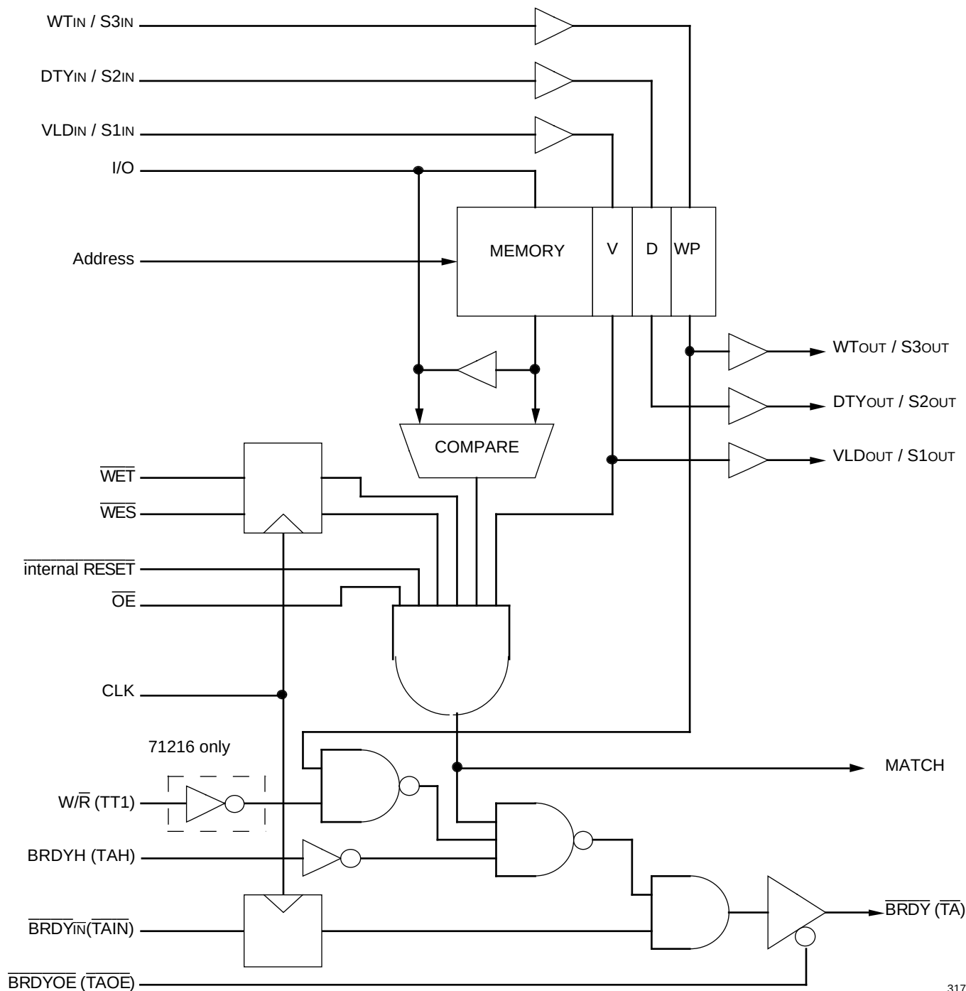
Figure 5. Dedicated Mode Logic (71216 pin names are in parenthesis)
