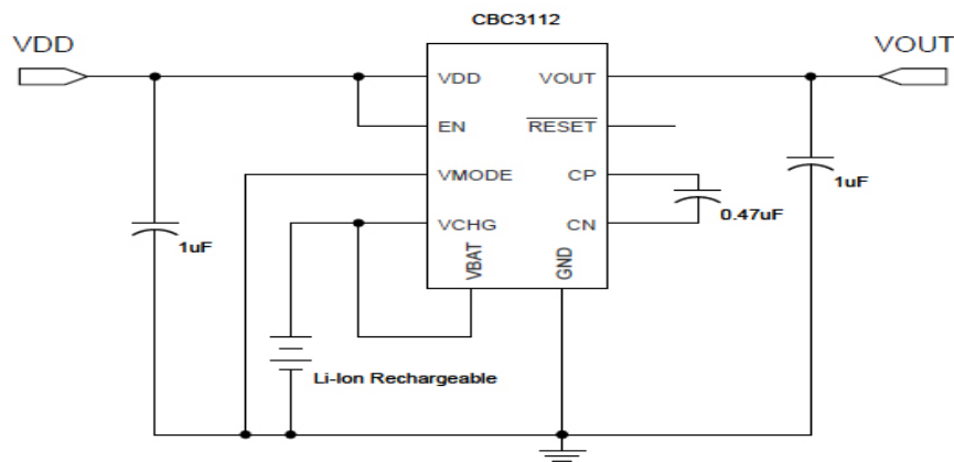
Figure 1: Application Circuit Showing Connection of External Li-Ion Rechargeable Cell.
