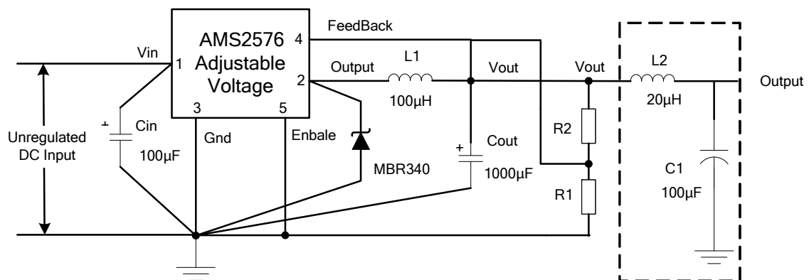
Figure 3: LC filter for Low Output Ripple
