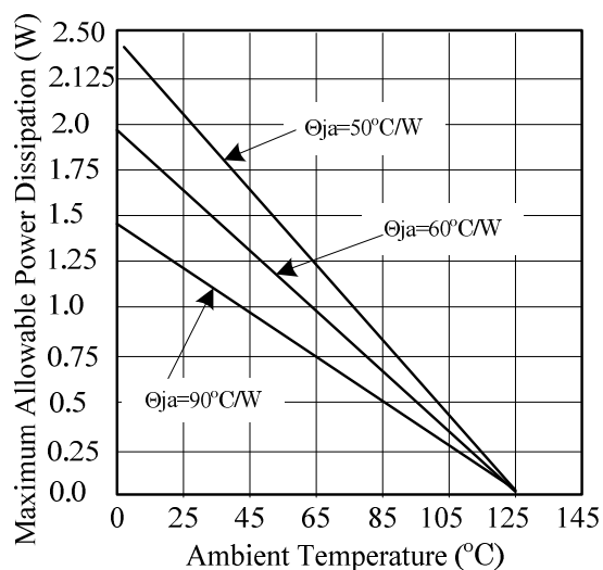
TO-252 Power Dissipation Still Air 20oz Cu on top Plane
